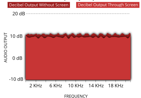
SAT-4K Frequency Response
